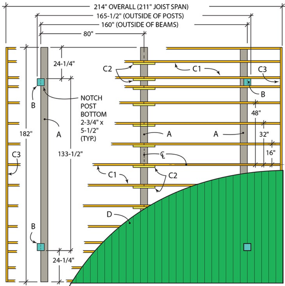
Fig. C Foundation Plan
