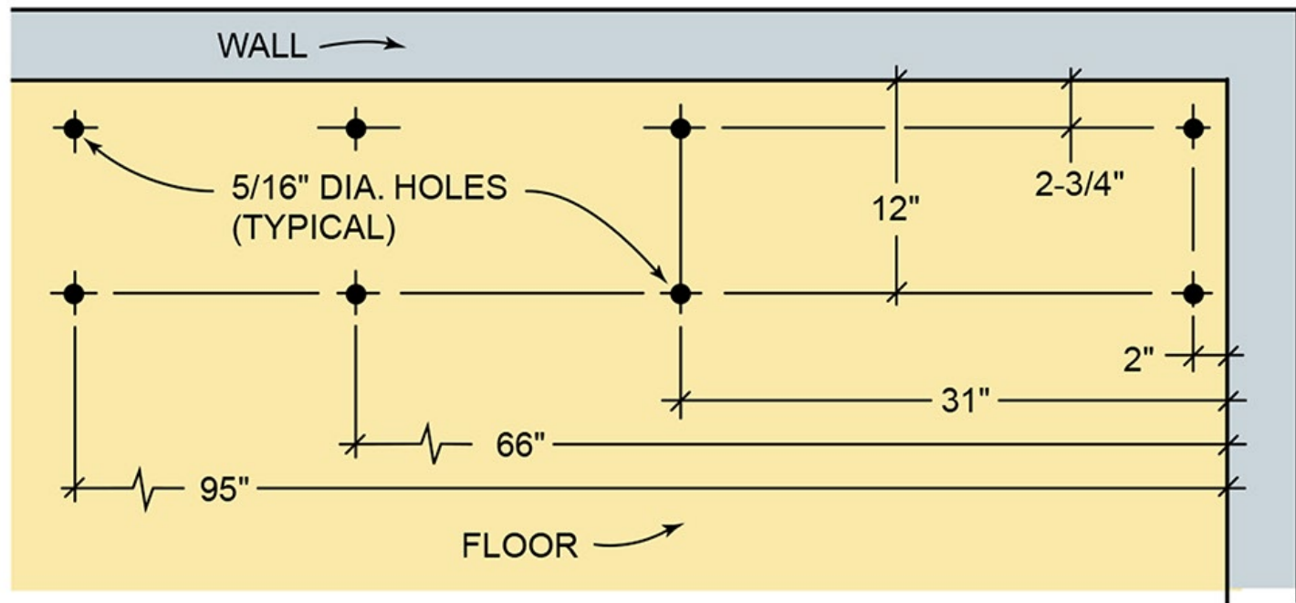
Fig. C Hole location for pins (top view)
