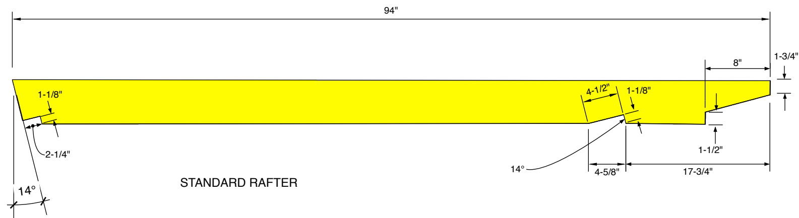
Figure G Rafter Details
