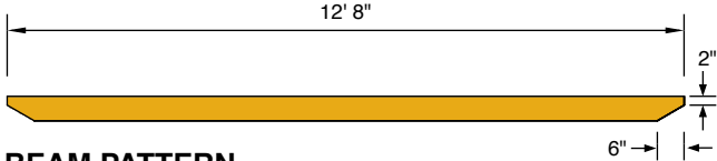
BEAM PATTERN
