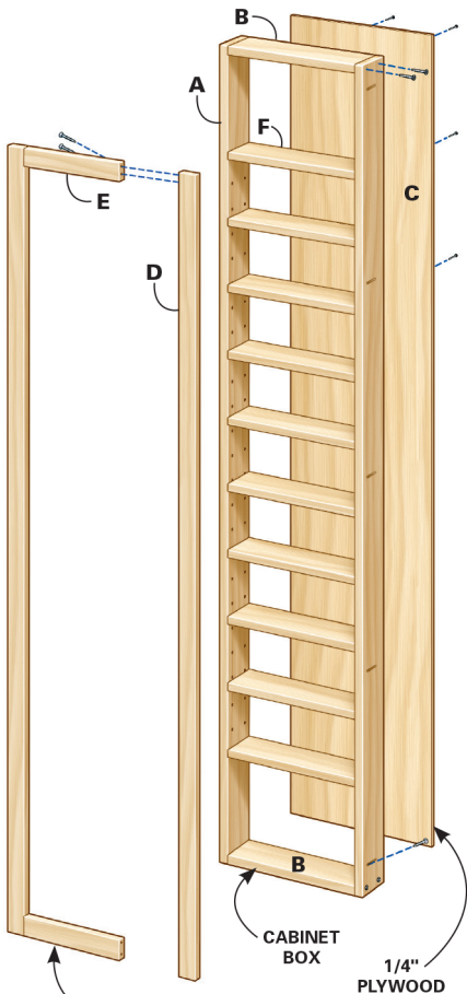
FACE FRAME 15-1/4" WIDE x 71-1/4" HIGH
