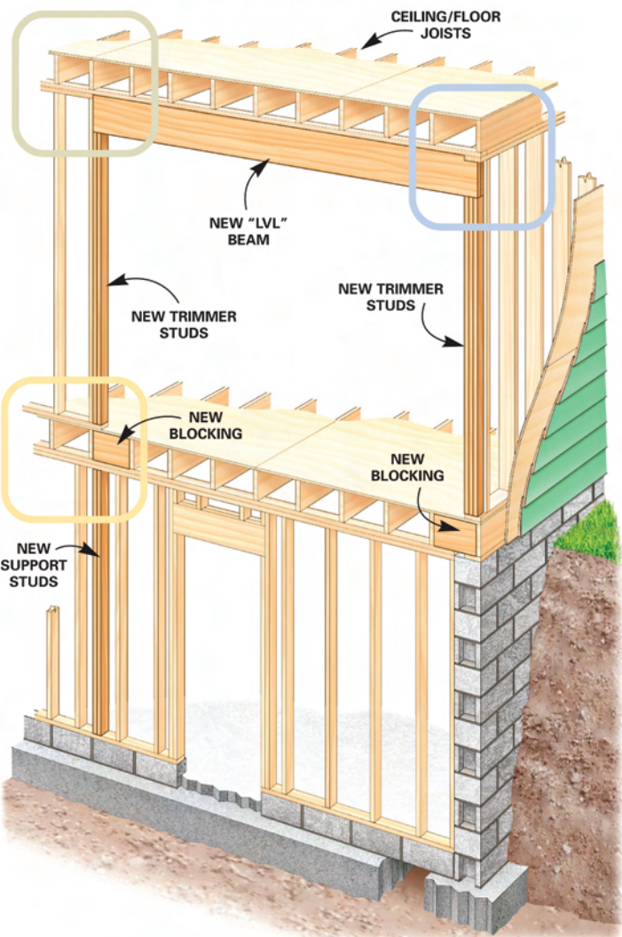
Figure A Bearing beam and support details
