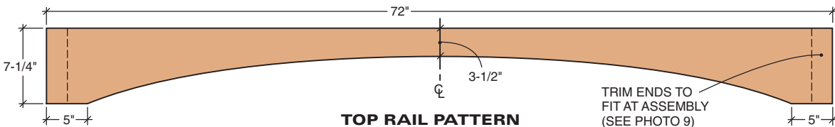
TOP RAIL PATTERN
