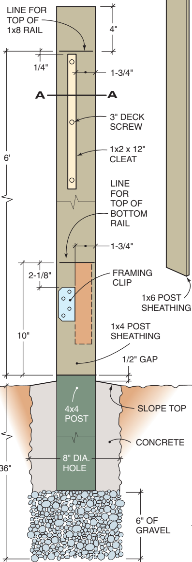
POST DETAIL
