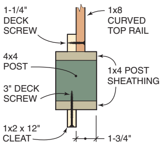
SECTION AT A
