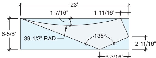
RAFTER TAIL EXTENSION DETAIL
