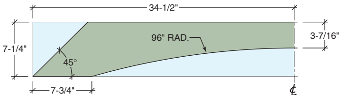
DECORATIVE COLLAR TIE DETAIL
