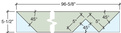
MAIN RAFTER DETAIL
