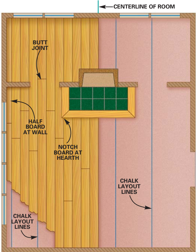
FLOOR LAYOUT PLAN
