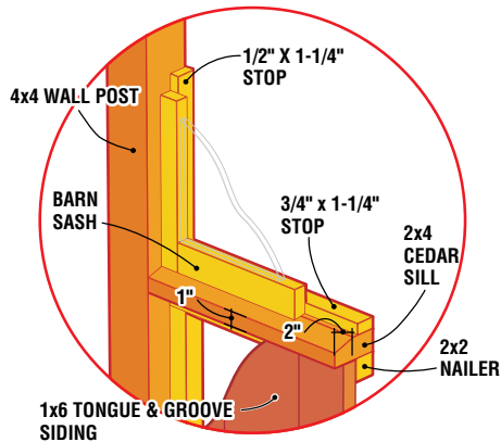
Fig. C Finish Details
