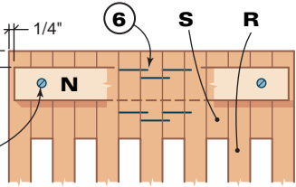
REMOVABLE GRATE
