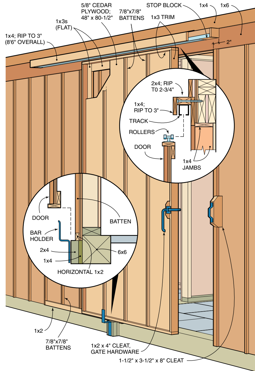
Figure G Sliding Door Detail
