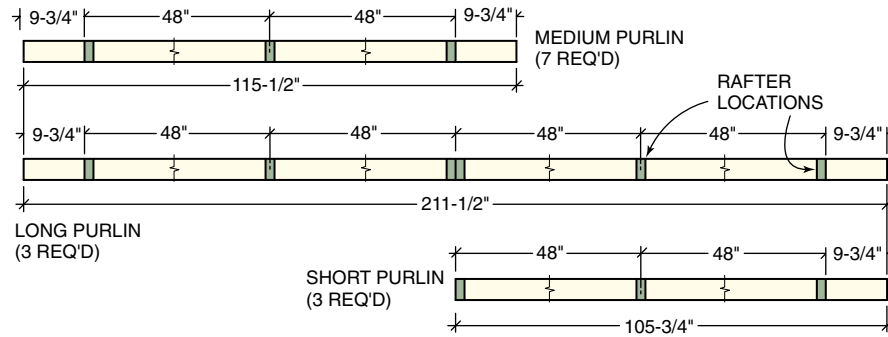
Figure E Purlin Details
