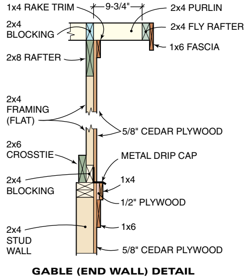
Figure F Gable and Eave Details
