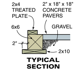
Figure B Foundation
