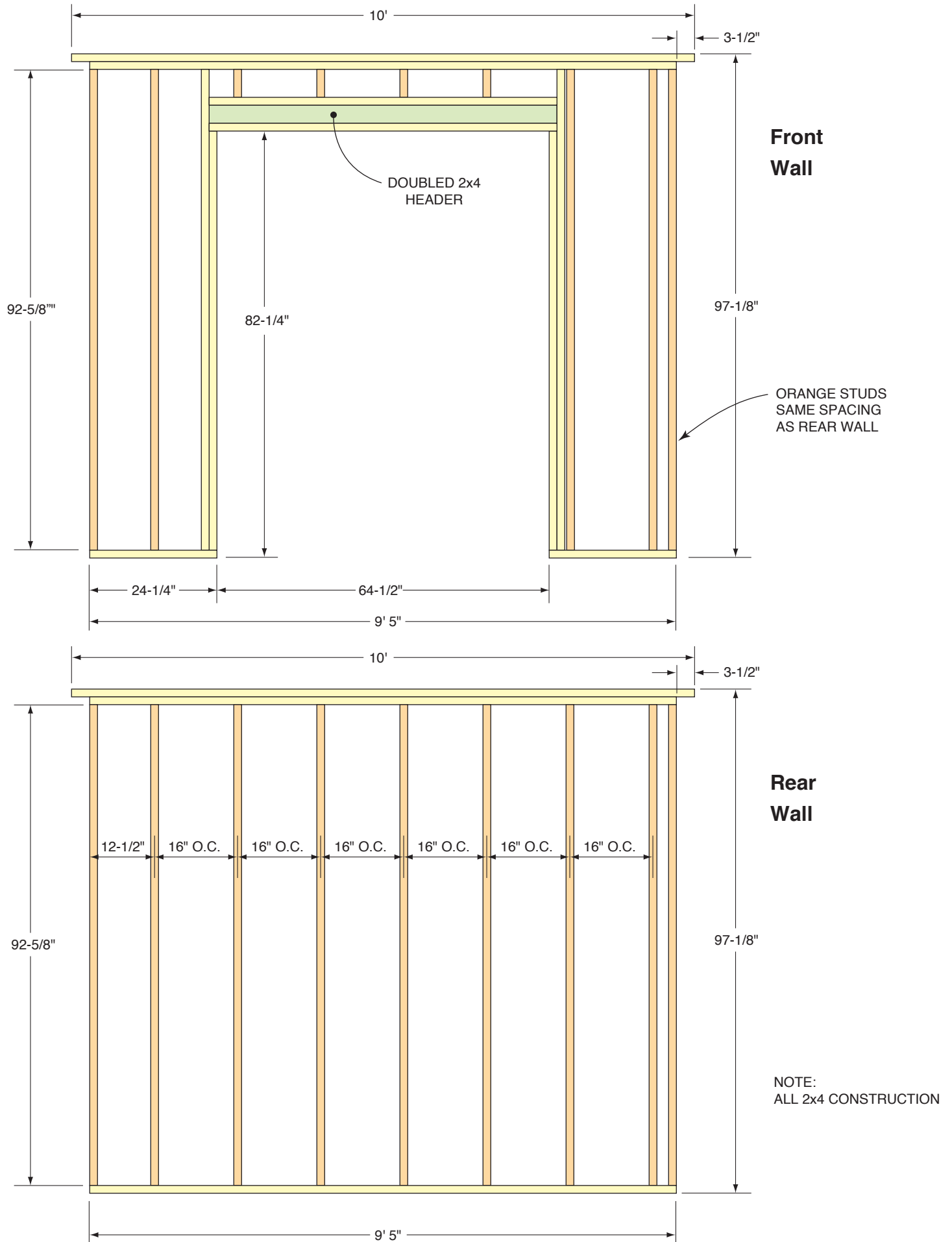
Front & Rear Walls Framing
