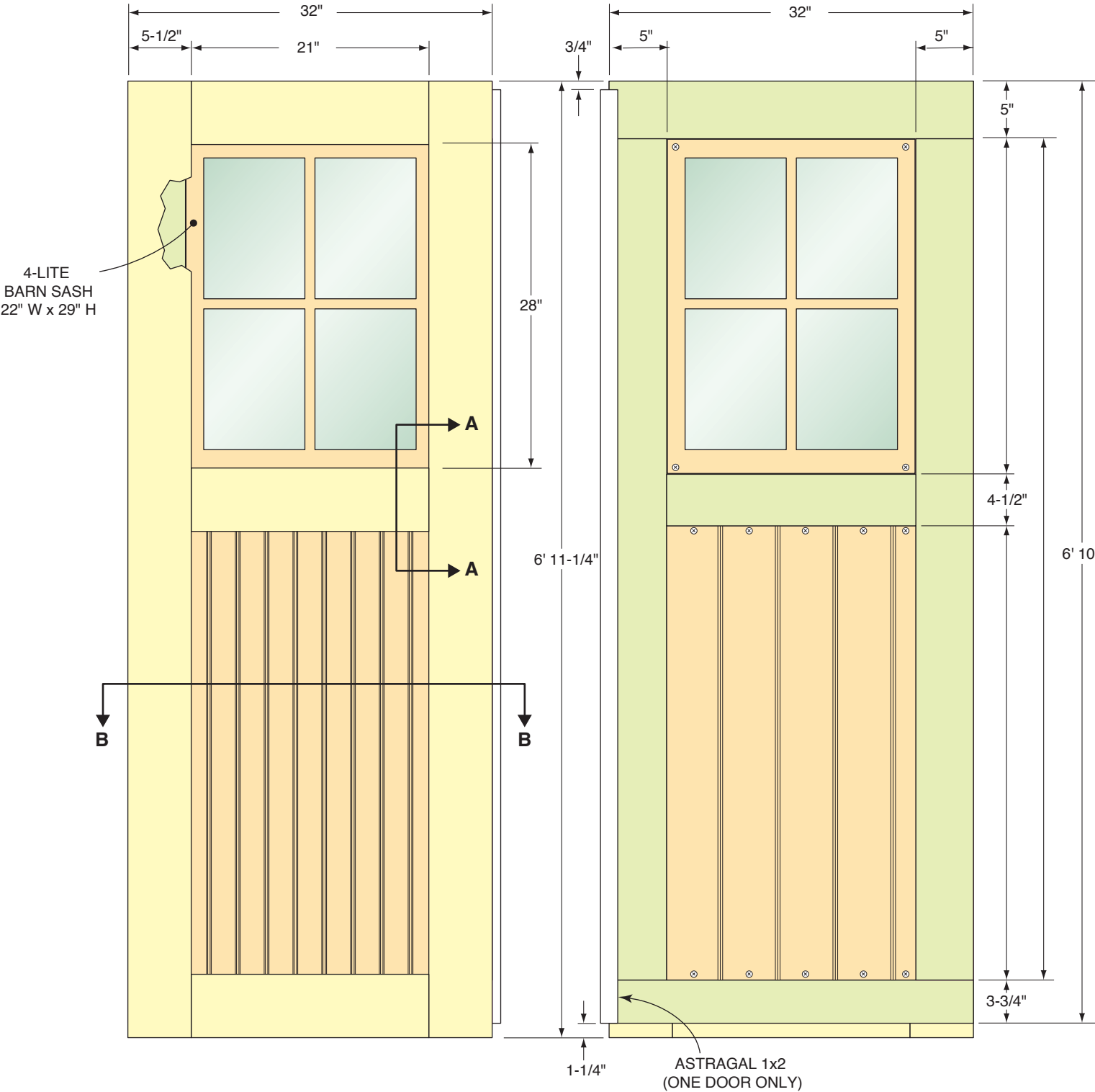
FRONT VIEW
