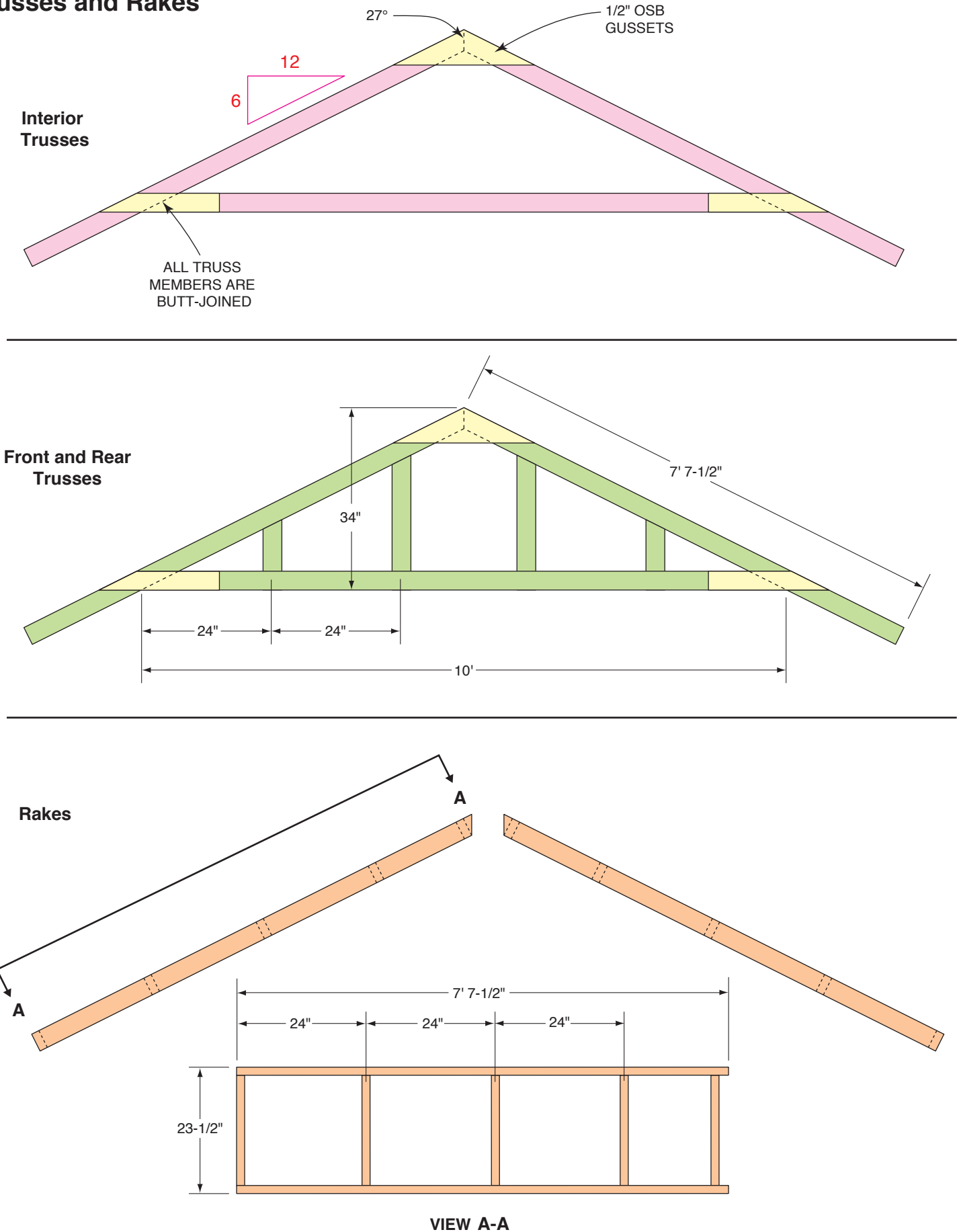
Figure G Trusses and Rakes
