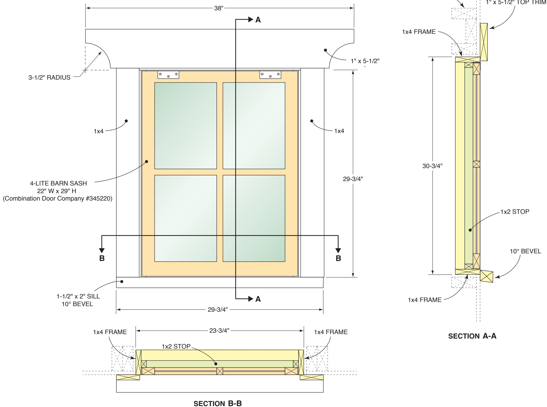
Figure M Site-Built Window
